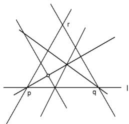
Figure 3: An illustration of the setup and conclusion of the Three Clause Lemma. The triangle T in the Lemma is the finite triangle \triangle(p, q, r) in the figure. The hollow vertex is the ordinary point attached to l in T guaranteed by the Lemma.
