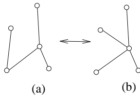
Figure 4: Transforming one tree into another takes only one flip optimally, but 5 flips through a canonical tree.
