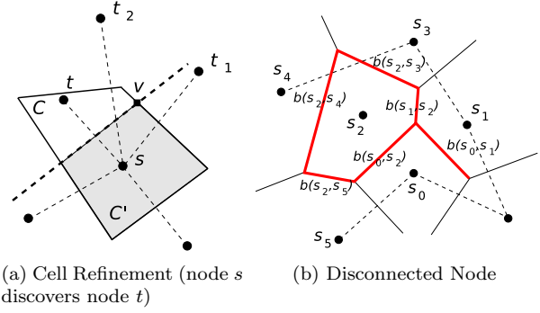
Figure 2: Illustration of the CC algorithm.
