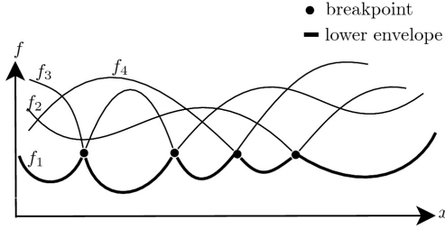
Figure 1: The lower envelope and its breakpoints
